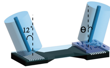
Fig. 6. Setup for fiber-to-chip measurement. The angle of the fiber at the left side is fixed at 12°, while the angle \theta of the fiber at the right-hand side can be changed from 0° to 24°.
