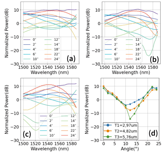
Fig. 7. Measurement results of normalized transmitted power for different number of LC layers (3, 5, and 7) as shown in (a), (b), and (c) respectively. Transmitted power for 1550 nm for layer count (3, 5, and 7) (d).
