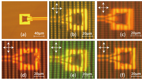
Fig. 4. Reflective optical microscope images of the grating couplers. The LC polymer in (a) is peeled off. Grating couplers in (b)-(f) are covered with 1, 3, 5, 7 and 9 spin-coated layers of LCPG, respectively.
