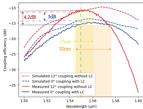
Fig. 8. Comparison of coupling efficiency between simulation and experimental data at 0^\circ and 12^\circ angles.
