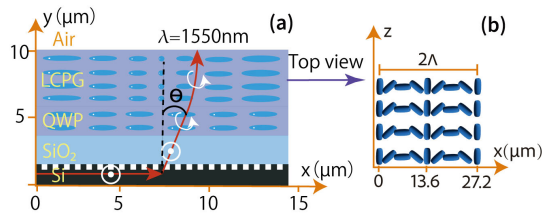
Fig. 1. Illustration of the cross section used for the FEM simulations (a). Top view of the orientation of the LC in the LCPG (b).
