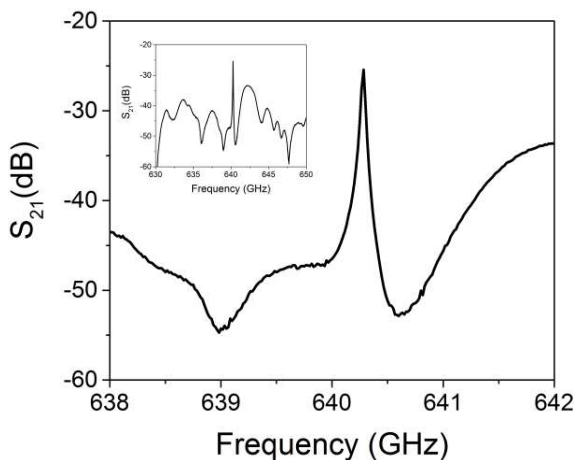
Fig. 18. Resonance frequency at f_R = 640.2 \text{ GHz} for cavity with N=25 hole. Inset: Zoom out of resonance plot
