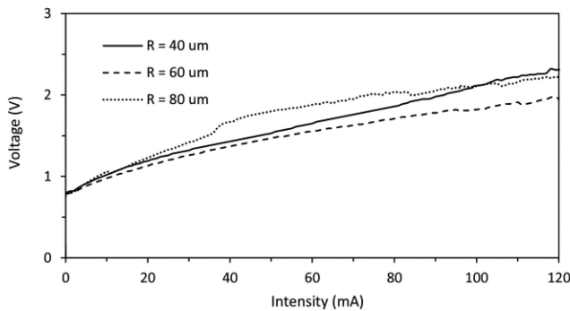
Fig. 3. V – I response of three microring diode lasers.
