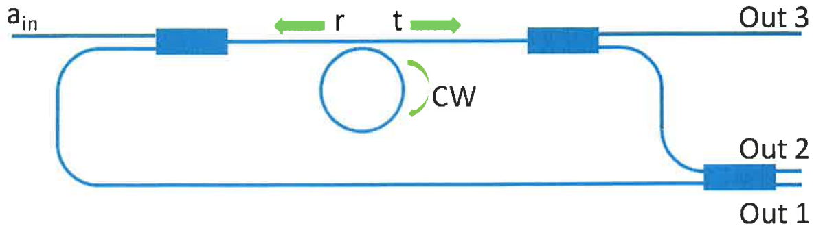
Figure 2: layout of the integrated interferometric circuit
