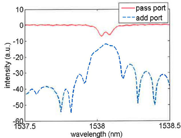
Figure 1: Measured spectra showing resonance splitting and backscattered power
