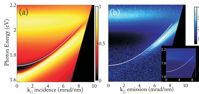
FIG. 2. (Color online) (a) Extinction and (b, main panel) PL enhancement angular spectra of p-polarized light of the sample described in the text. PL enhancement of s-polarized light is shown in the inset of (b). The white lines indicate the degenerate (\pm 1, 0) Rayleigh anomalies.
