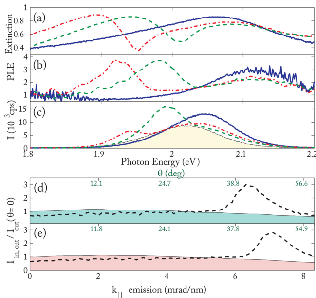
FIG. 3. (Color online) (a) Extinction, (b) PL enhancement, and (c) emission inside the array, i.e., I_{in} , in 10^3 counts per second, at k_{||} = 0 (blue solid lines), k_{||} = 7 mrad/nm (red dashed-dotted lines), and k_{||} = 7.9 mrad/nm (green dashed lines). The filled area in (c) is the emission outside the array, i.e., I_{out} , at k_{||} = 0 ; I_{out} for the larger values of k_{||} (not shown here) has the same line shape as in k_{||} = 0 , but with a lower amplitude. (d) and (e) show the angular dependent emission for an energy of (d) 1.89 eV, and (e) 1.93 eV, with I_{in} as black dashed lines and I_{out} as a filled area. Both I_{in} and I_{out} are normalized to the value of I_{out} at \theta = 0 for each energy. The upper ticks indicate the value of the emission angle \theta corresponding to the k_{||} values in the x-axis. All measurements are shown for p-polarized light.
