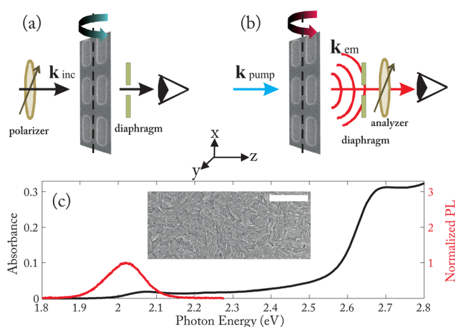
FIG. 1. (Color online) Setup used for (a) extinction and (b) PL enhancement measurements. The sample is represented by a SEM image of a silver nanoantenna array, with the dashed lines indicating the axis of rotation for the sample in (a) and detector in (b). (c) Absorbance (left axis) and normalized PL (right axis) of CdSe/CdS core/shell quantum rods (QRs). The inset in (c) shows a SEM image of a spin-coated layer of QRs; the scale bar denotes 200 nm.
