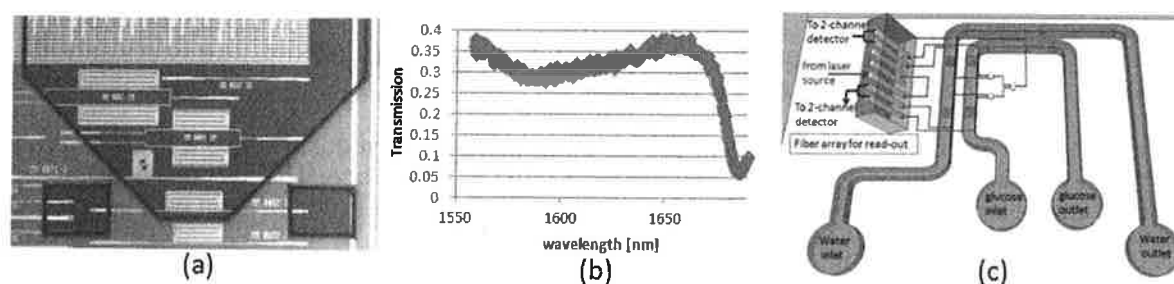
Figure 1. (a) Fabricated SOI spiral with SU8 box (b) Transmission spectrum of IPA (c) Sensor with microfluidics
