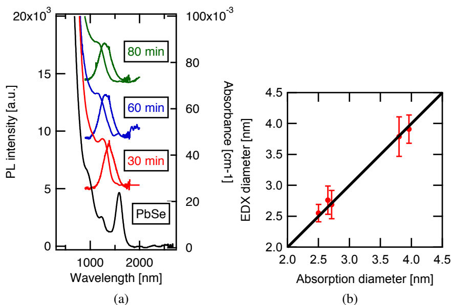
Figure 2: (a) Absorption and luminescence spectra of PbSe/CdSe QDs in C_2Cl_4 for increasing exchange times. (b) Diameter determined from EDX vs. diameter determined from the position of the first absorption peak, using the PbSe sizing curve. The black line indicates a 1-to-1 relationship. 12
