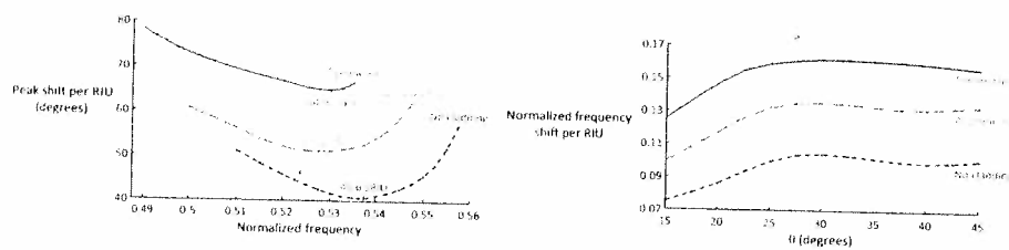
Figure 3: As expected, the shift for the symmetric cladding configuration is the highest in both approaches (left: monitoring the angular shift at a fixed frequency; right: measuring the frequency shift at a fixed angle).
