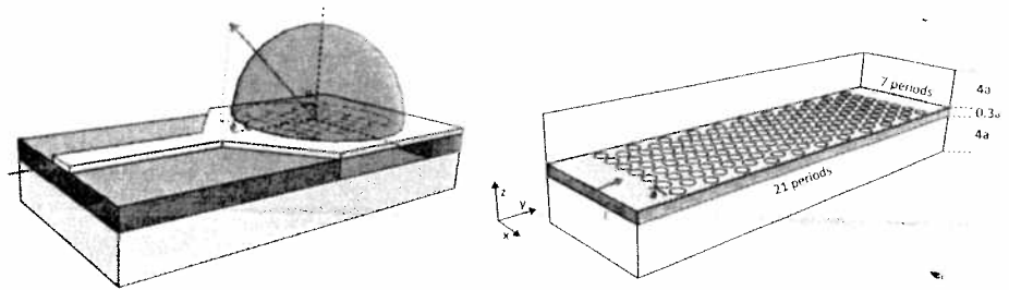
Figure 1: Light enters the PhC biosensor through a waveguide and is coupled to free space as a beam with inclination \theta and azimuth \phi (left). The simulated structure used for FDTD simulations is shown in the right figure. All sizes are normalized to the lattice constant a .
