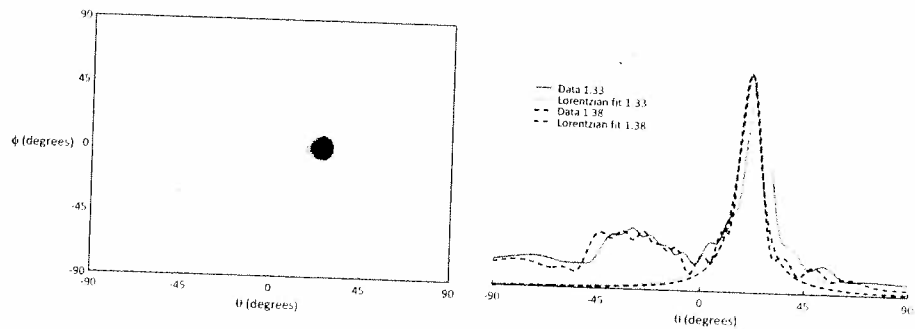
Figure 2: The angular spectrum (left) and cross-section at \phi=0^\circ (right) of the vertically projected Poynting vector of the proposed structure with a symmetric cladding (i.e. refractive index above and below PhC slab equals that of the holes) at normalized frequency 0.53488. A Lorentzian resonance shape is clearly visible.
