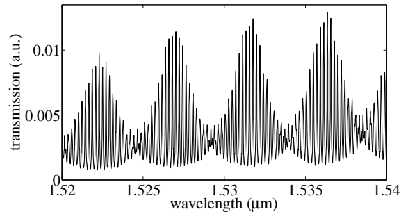
Fig. 4. Measured transmission spectrum of the device as deionized water is flowing over the sensor ring resonator. The height of the envelope peaks varies due to the wavelength-dependent coupling efficiency of the grating couplers.
