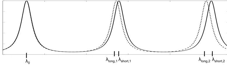
Fig. 7. Transmission spectra of the two individual ring resonators with different optical roundtrip. The resonator with the short optical roundtrip (solid line) has a larger free spectral range than the resonator with the long optical roundtrip (dashed line).
