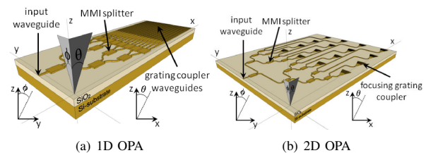
Fig. 2. Optical phased arrays fabricated on silicon-on-insulator.
