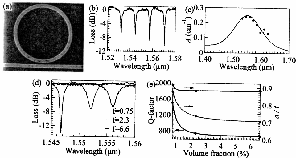
Figure 3: (a) SEM image of a SOI notch filter. (b) Transmission spectrum for a Q-PbSe coated ring. (c) Comparison of the absorption coefficient of the ring ( -2\log a ) with the Q-PbSe absorption coefficient. (d) Transmission spectra for Q-PbS coated rings with varying Q-PbS volume fraction f . A shift to higher wavelengths is observed with increasing f due to the increase in the effective refractive index. (e) The Q-factor decreases with increasing f (black dots). This is due to an decrease in a (blue), as t remains fairly constant (red).
