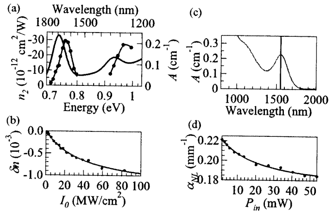
Figure 2: (a) n_2 -spectrum (blue) compared to the absorbance spectrum (black). (b) Intensity dependence of \delta n . A clear saturation is observed. (c) Q-PbS Absorbance spectrum of particles with a peak absorption at 1.55 \mu\text{m} . (d) The nonlinear absorption coefficient \alpha_{NL} at 1.55 \mu\text{m} decreases with increasing optical intensity.
